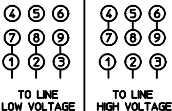
WIRING DIAGRAM
