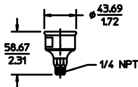
MUFFLER ASM. (SHIPPED UNATTACHED)
