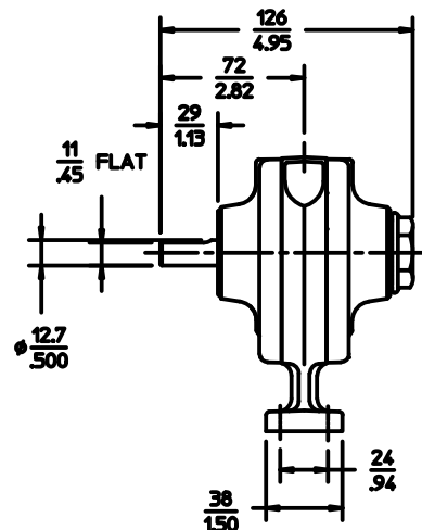
MUFFLER ASM. (SHIPPED UNATTACHED)
