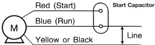
< MOTOR WITH 3 LEADS & CAPACITOR
